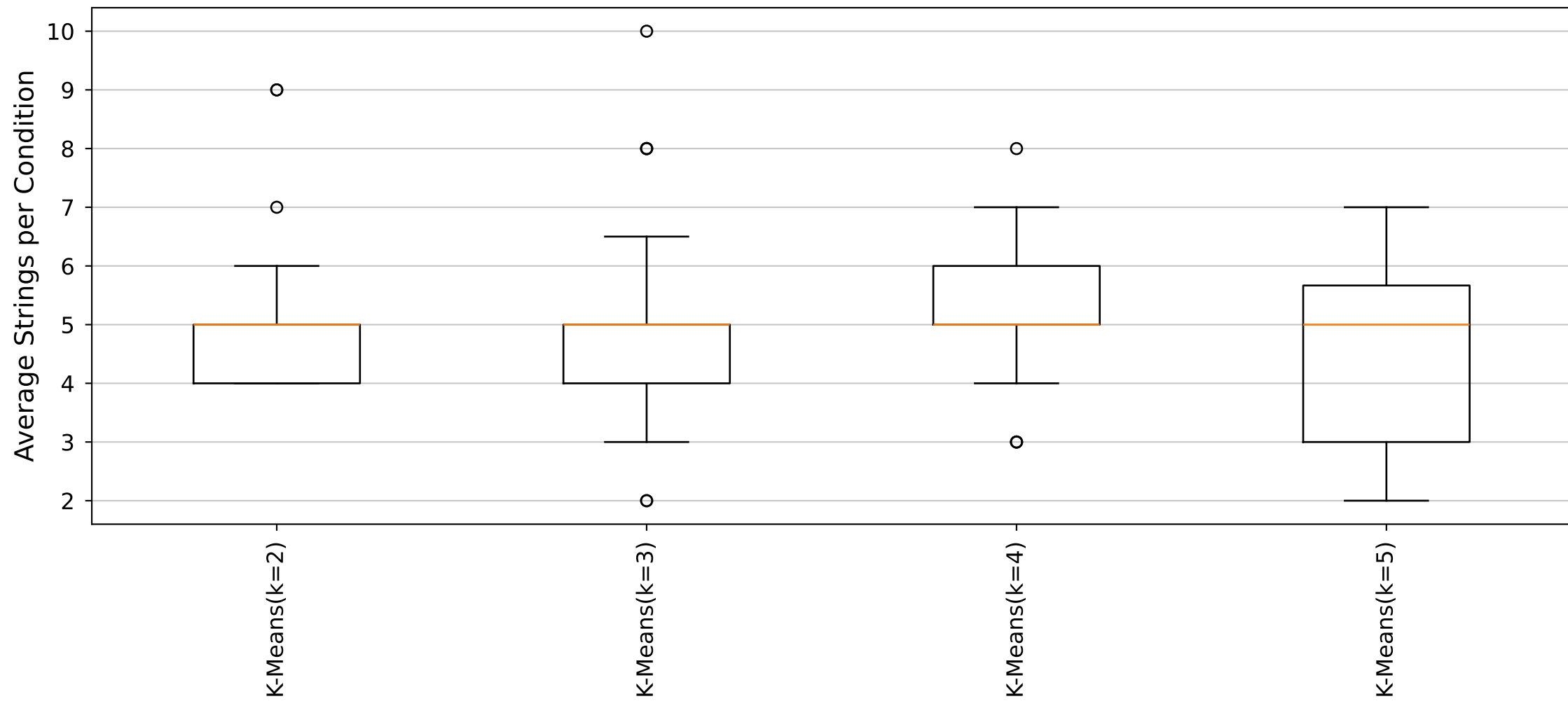
YARA Rules Average Strings per Condition Distribution (Cluster35_Size5 dataset)
